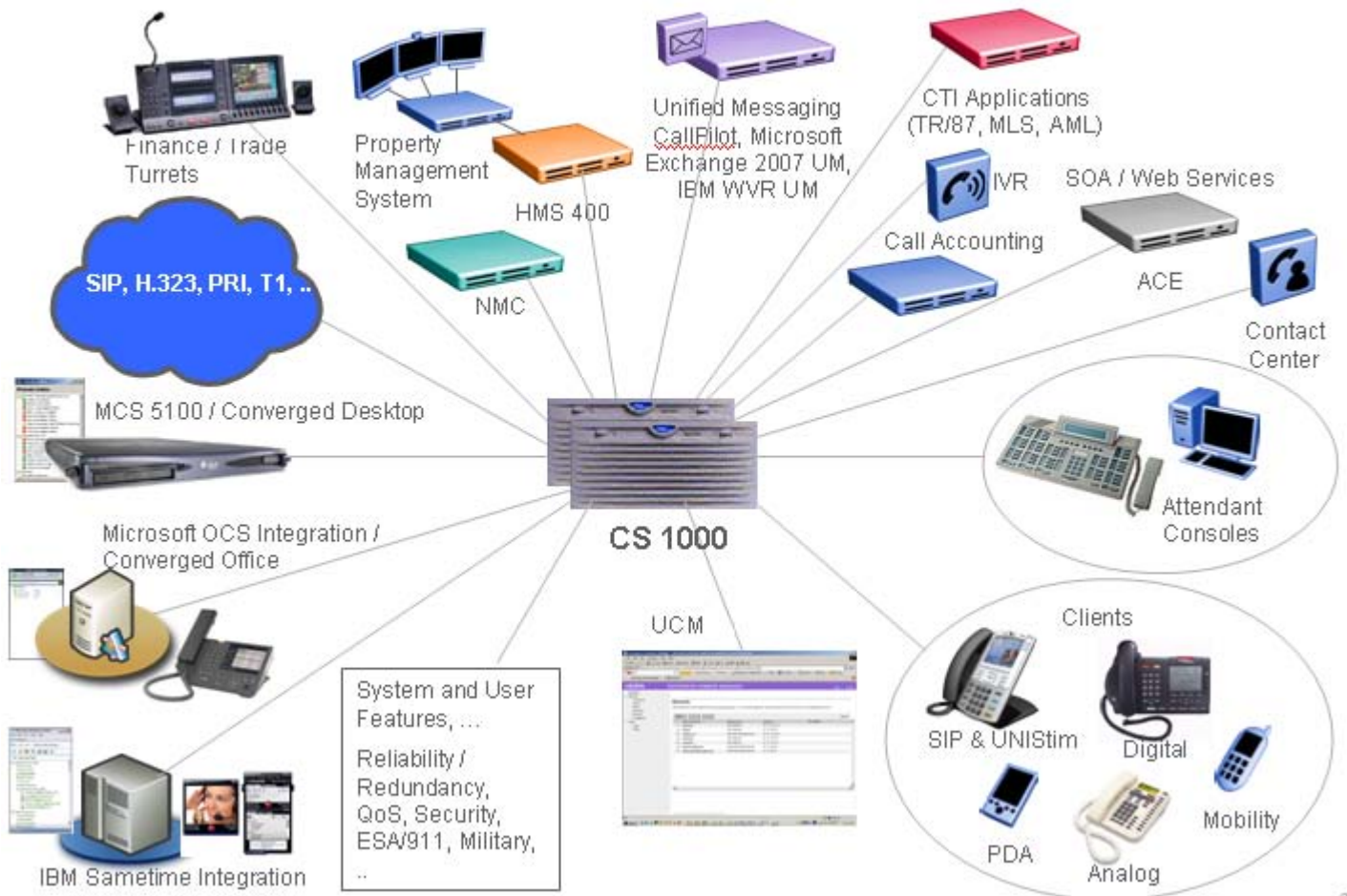
Figure 1: System architecture
