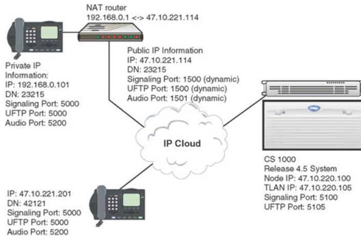
Figure 19: Using NAT with UFTP
