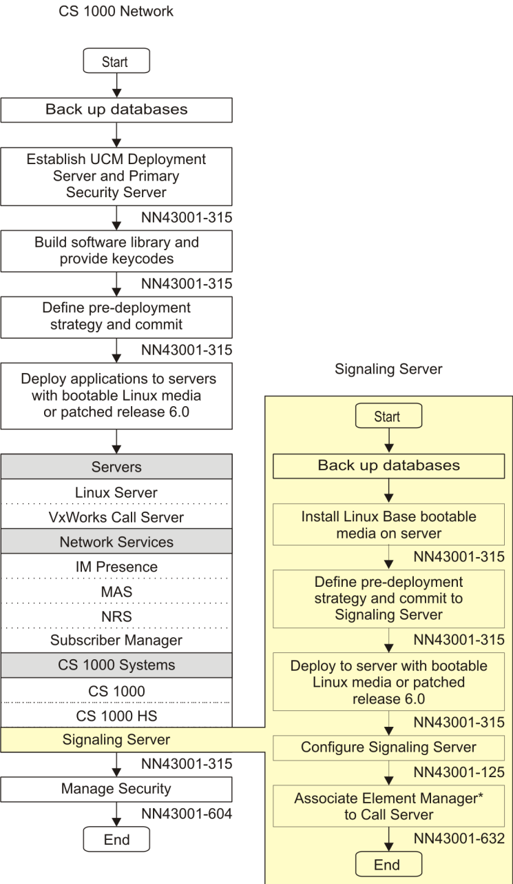
Figure 42: Linux base and applications installation task flow
