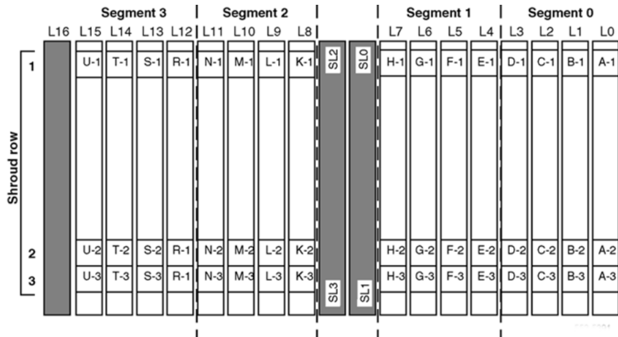
Figure 121: Backplane slot designations
