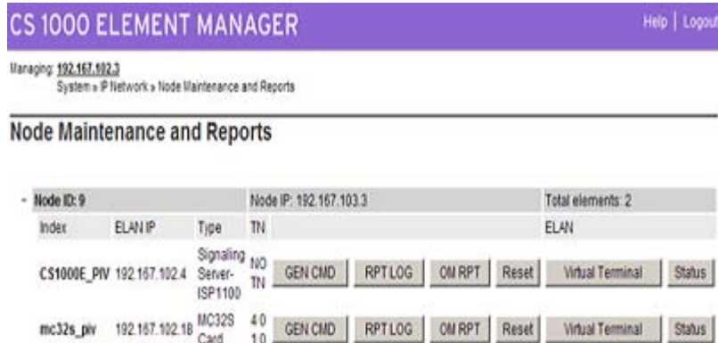
Figure 86: Voice Gateway Media Card and GEN CMD button
