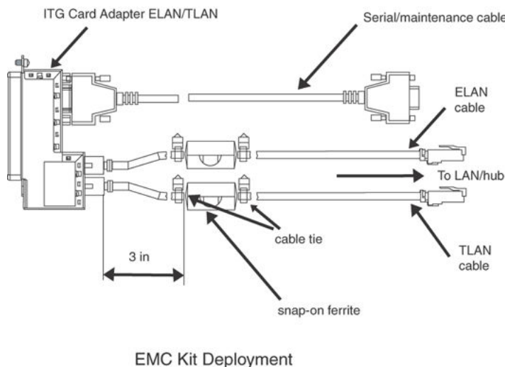
Figure 57: ITG EMC Shielding Kit Deployment
