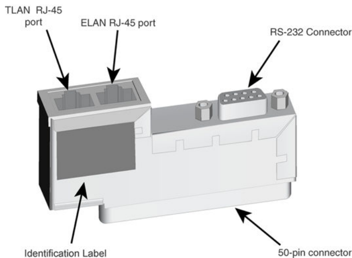
Figure 56: Shielded 50-pin to Serial/ELAN/TLAN Adapter
