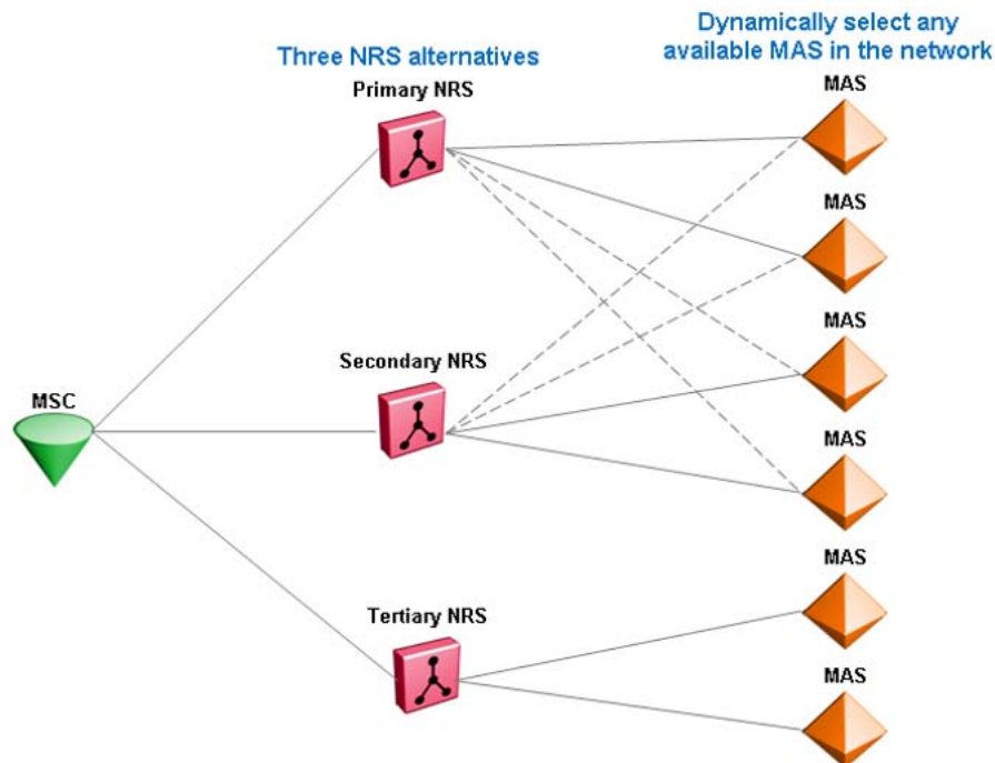
Figure 94: Alternate NRS routing
