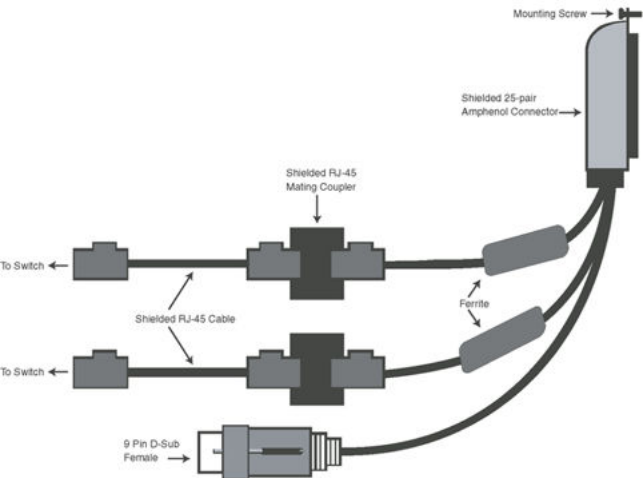
Figure 118: NTMF94EA ELAN, TLAN and RS-232 serial maintenance I/O cable
